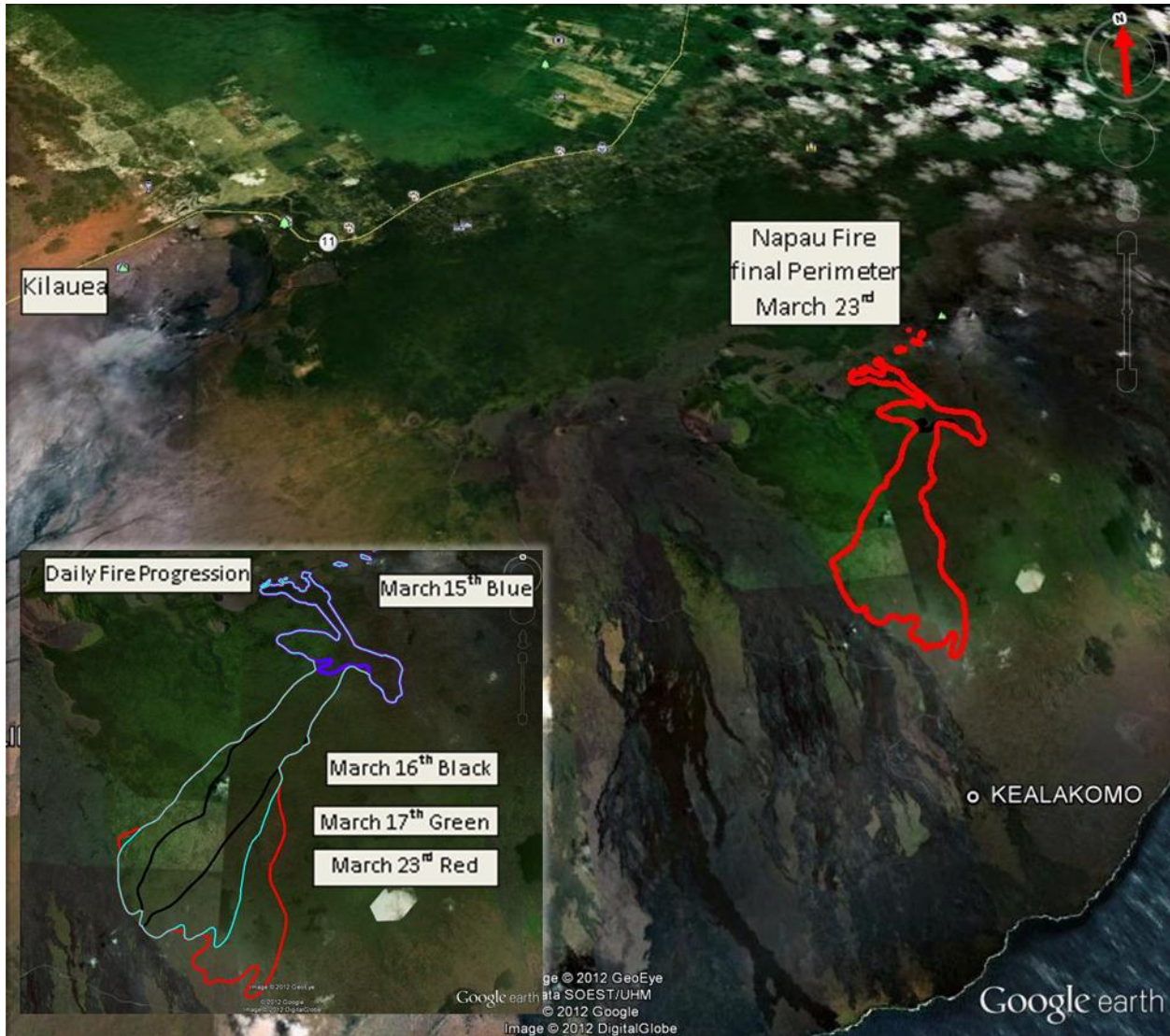
Figure 18 - Overview of Napau Fire March 2011. The fire extended nearly 4 miles in length depicted by the black line.
